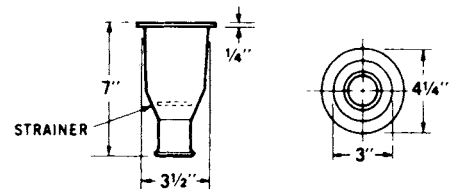
FIG. 42 Beaded Outlet 3-in. Hemispherical
