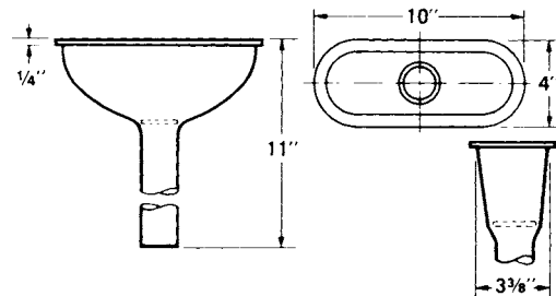
FIG. 41 Plain End Outlet 3- by 9-in. Oval
