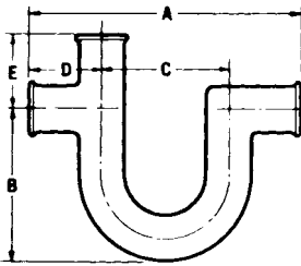
FIG. 26 Running Trap (Vented)
