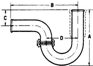
FIG. 22 Running Trap
