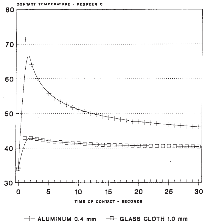
LIGHT DENSITY FIBEROUS GLASS INSULATION CONTACT TEMPERATURE AT 0.08 mm DEPTH
