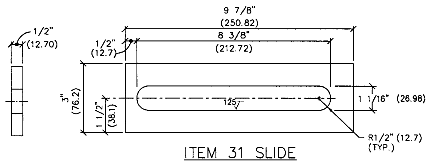
FIG. 4 Detail Drawings of Bond Wrench (continued)
