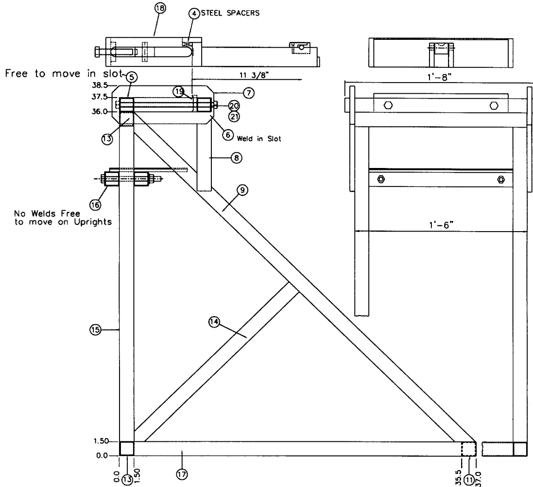
FIG. 2 Bond Wrench Frame and Elevation
