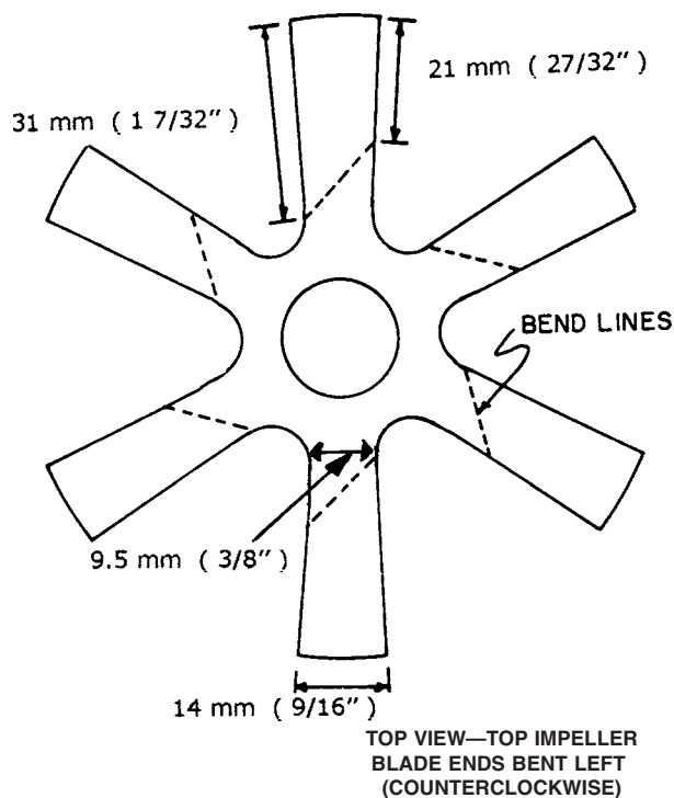
Impeller—102 mm (4 in.) diameter × 1.5 mm (No. 16 gage) thick; Three Layers Shaft—19 mm (3/4 in.) diameter extending 9.5 mm (3/8 in.) below bottom layer and the ends of the blades bent to 45° pitch. Blades on the top and bottom layer bent to the left (counterclockwise) and the middle layer bent to the right (clockwise).
