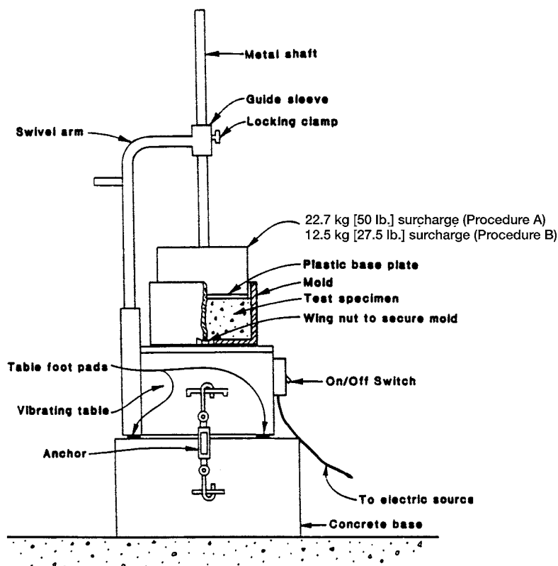
FIG. 1 Vibrating Table—Consistency Test
