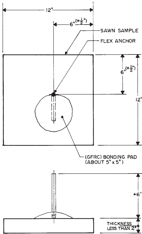
FIG. 4 Test Specimen
