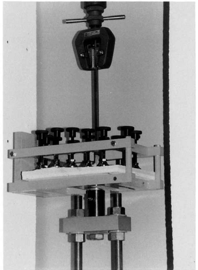
FIG. 3 Suitable Test Fixture
