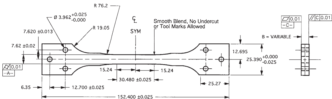
NOTE: 1) SURFACE FINISH 0.5- 1.0 µm ALL OVER EXCEPT END FACES WHICH MAY BE 1.0-2.0 µm. 2) FINAL GRIND OF GAGE SECTION TO BE LONGITUDINAL FIG. 15 Example of a Contoured, Pin/Face-Loaded Test Specimen Geometry (4)
