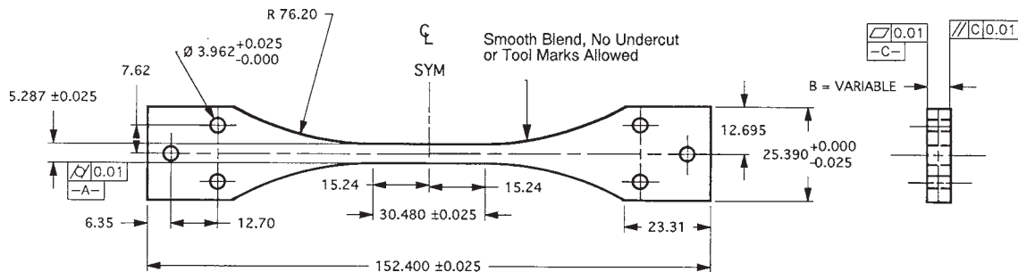
FIG. 13 Example of a Beveled Tab Successfully Used with Face-Loaded CFCC Tensile Test Specimens (11)
