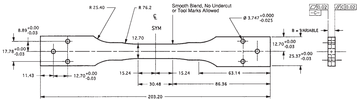
NOTE: 1) SURFACE FINISH 0.5- 1.0 µm ALL OVER EXCEPT END FACES WHICH MAY BE 1.0-2.0 µm. 2) FINAL GRIND OF GAGE SECTION TO BE LONGITUDINAL FIG. 16 Example of a Contoured, Pin/Face-Loaded Test Specimen Geometry (5)
