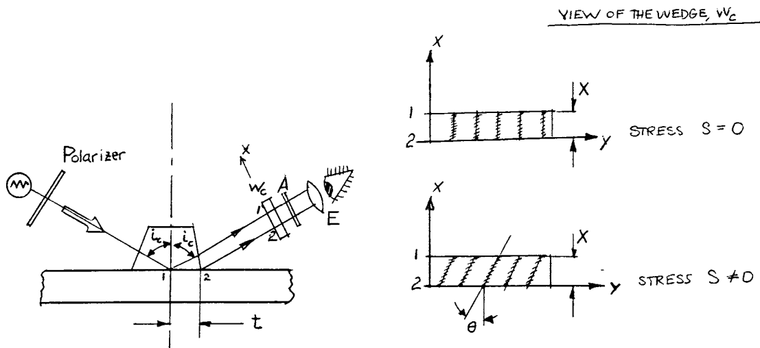
FIG. 1 Apparatus For Measuring Surface Stress
