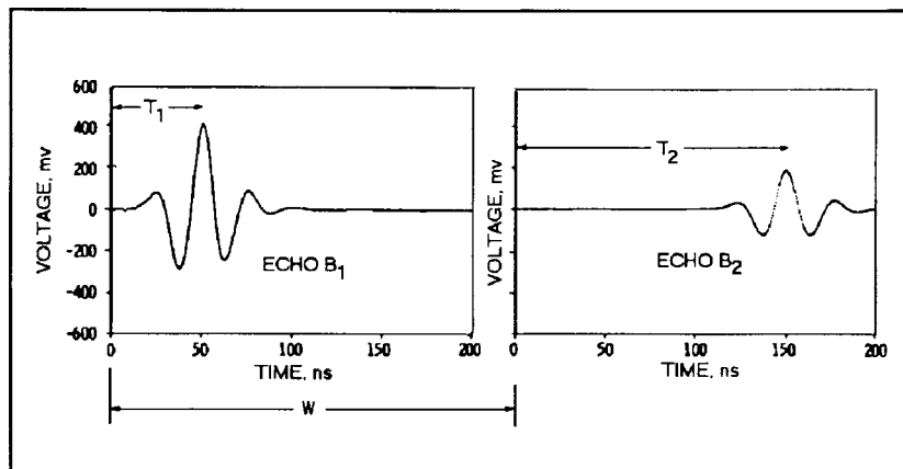
NOTE 1—Time delay, W , between the two window start times is predetermined. Time interval, T , between echoes B_1 and B_2 is calculated from T = W + (T_2 - T_1) .
