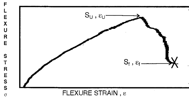
c) Stress-Strain Curve with a Nonlinear Region
