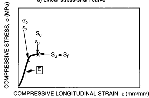
b) Stress-strain curve with a linear region followed by decreasing stiffness
