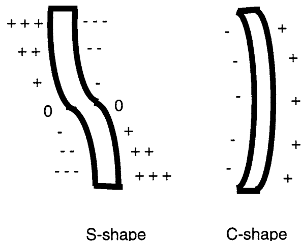
FIG. X1.2 S-Shape and C-Shape Bending of Compressive Test Specimen
