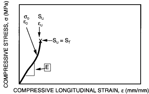
c) Stress-strain curve with a linear region followed by increasing stiffness
