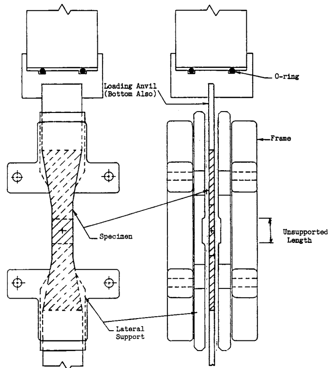
FIG. 4 Example of a Controlled Face Supported Fixture (4)
