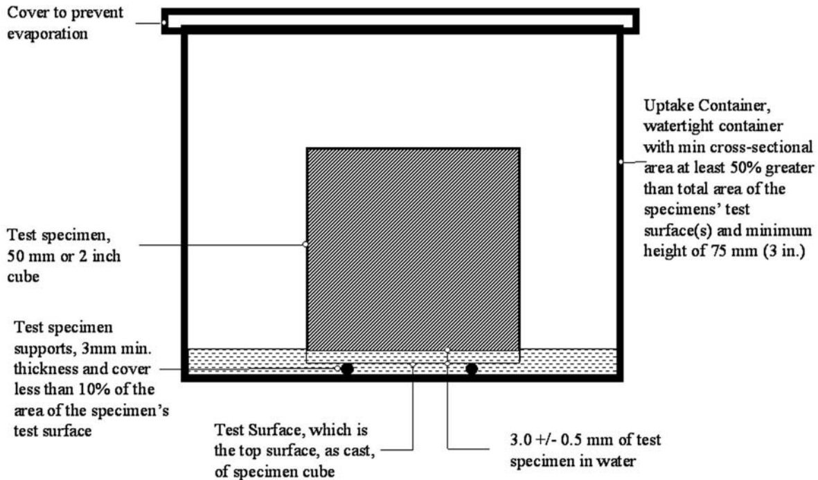
FIG. 1 Specimen Configuration During Testing
