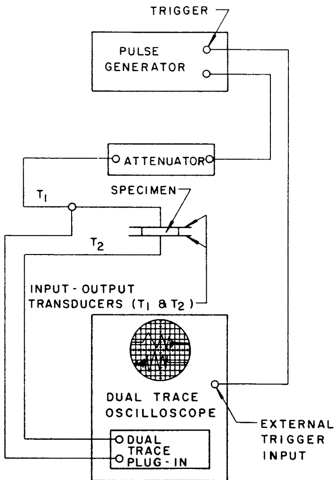
FIG. 1 Equipment Set-up
