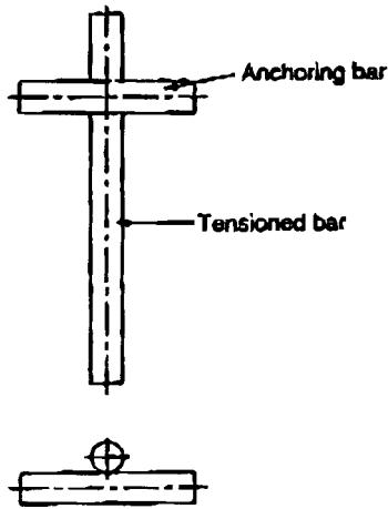
FIG. 2 Weld-Point Shear Strength Test Specimens
