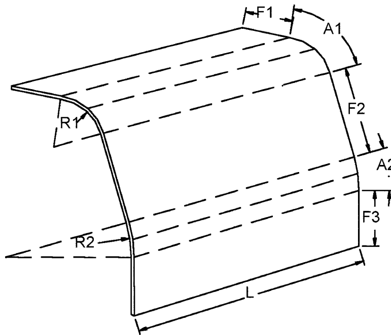
FIG. 2 Single Bend
