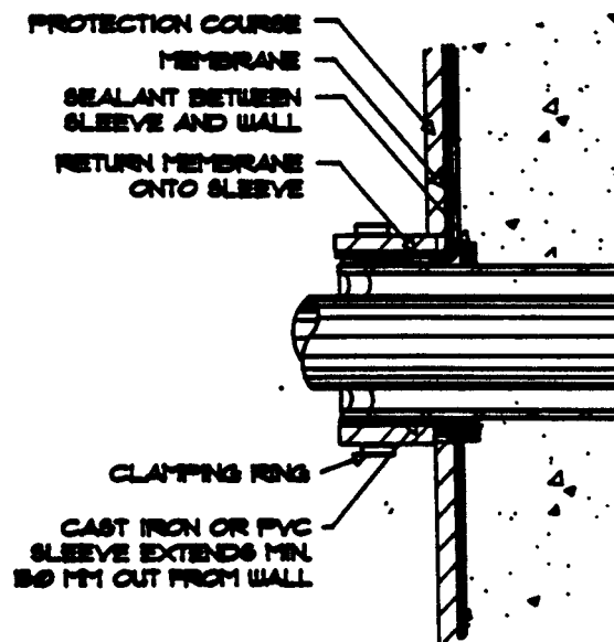
FIG. 3 Pipe Penetration
