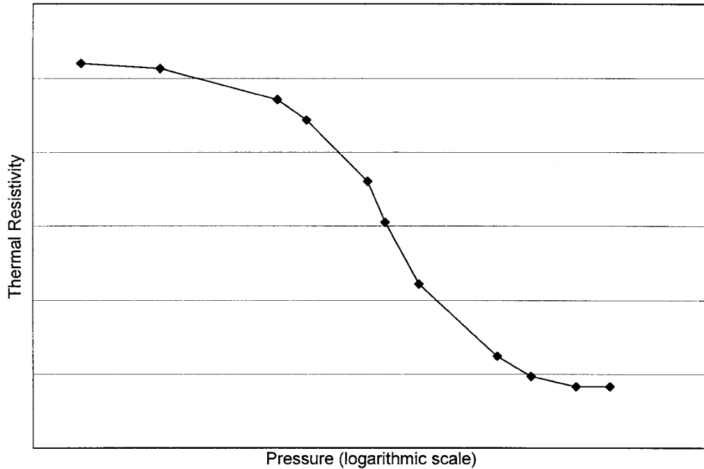
FIG. X1.1 Typical Relationship Between Center-of-Panel Thermal Resistivity and Internal Panel Pressure
