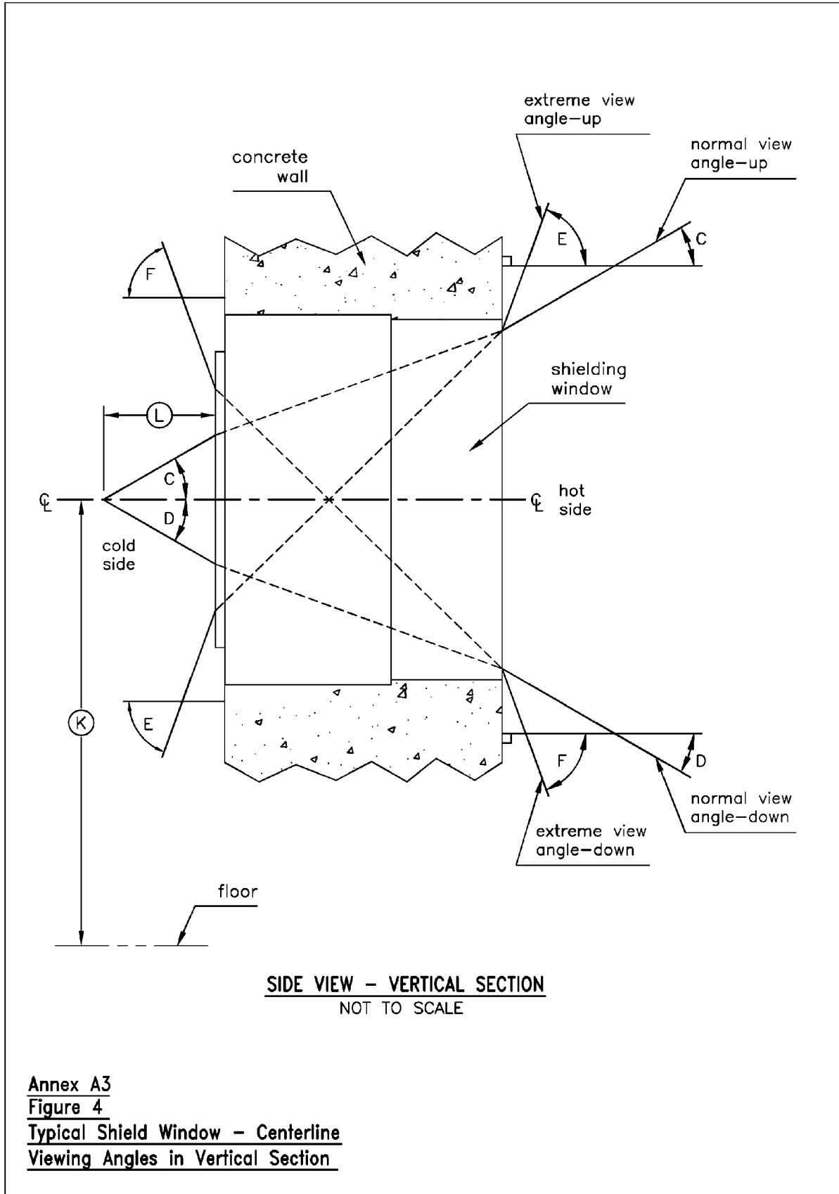
FIG. A3.4 Typical Shield Window—Centerline Viewing Angles in Vertical Section
