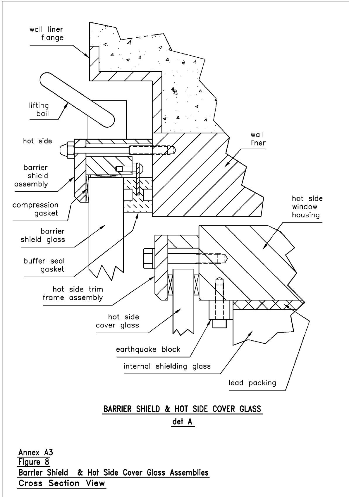
FIG. A3.8 Barrier Shield and Hot Side Cover Glass Assemblies—Cross Section View
