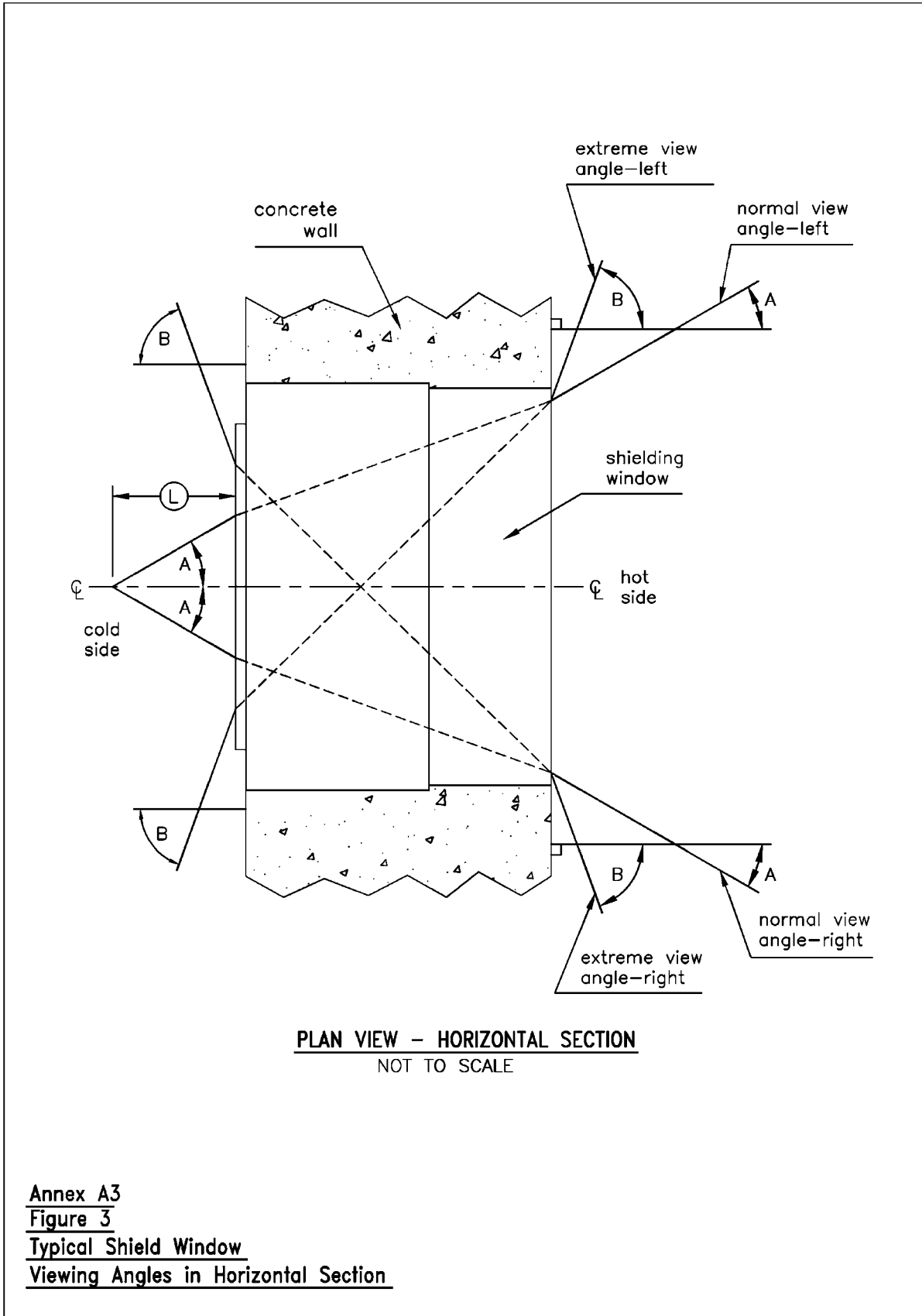
FIG. A3.3 Typical Shield Window—Viewing Angles in Horizontal Section
