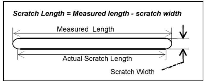
FIG. A2.1 Schematic for Scratch Length Measurement
