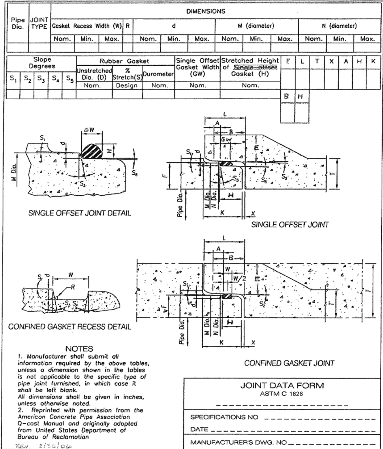
FIG. X2.1 ASTM Joint Dimension Data
