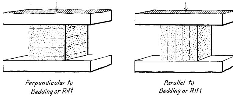
NOTE 1—Dashed lines indicate direction of bedding or rift. Arrows indicate direction of loading. (a) Loading Perpendicular to Bedding or Rift (b) Loading Parallel to Bedding or Rift
