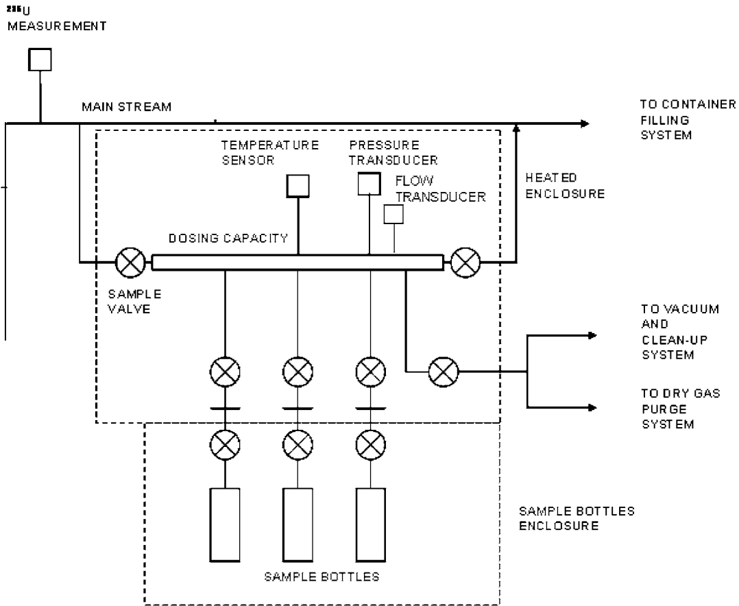
FIG. 2 Schematic Arrangement for Sampling According to Practice 2
