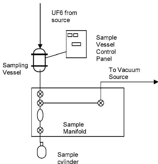
FIG. 1 Schematic Arrangement for Sampling According to Practice 1
