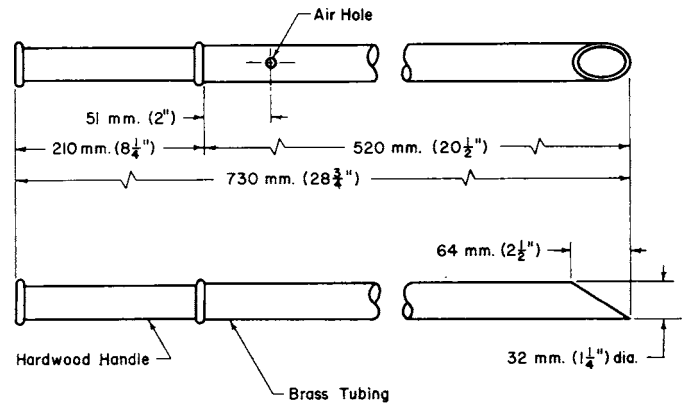
FIG. 2 Tube Sampler for Packaged Cement
