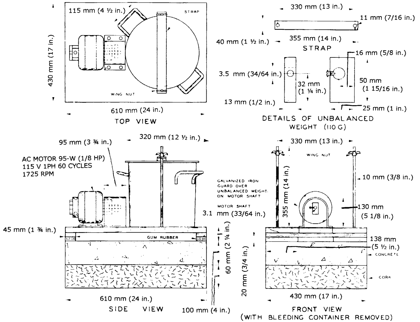
FIG. 2 Detail of Vibrating Platform Apparatus
