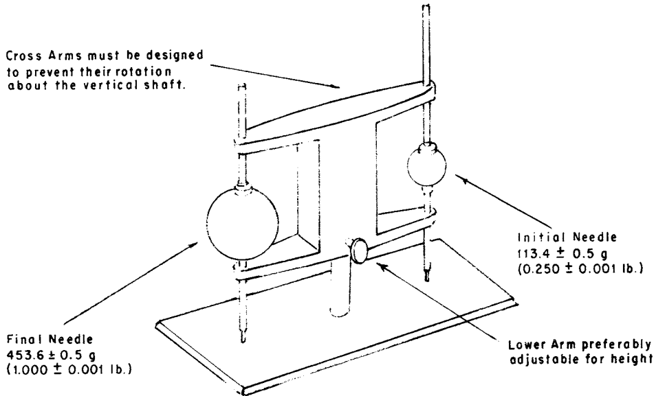
(b) Gillmore Apparatus
