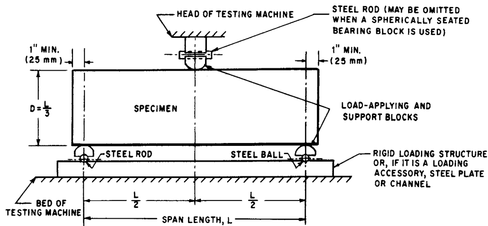
FIG. 1 Diagrammatic View of a Suitable Apparatus for Flexure Test of Concrete by Center-Point Loading Method.
