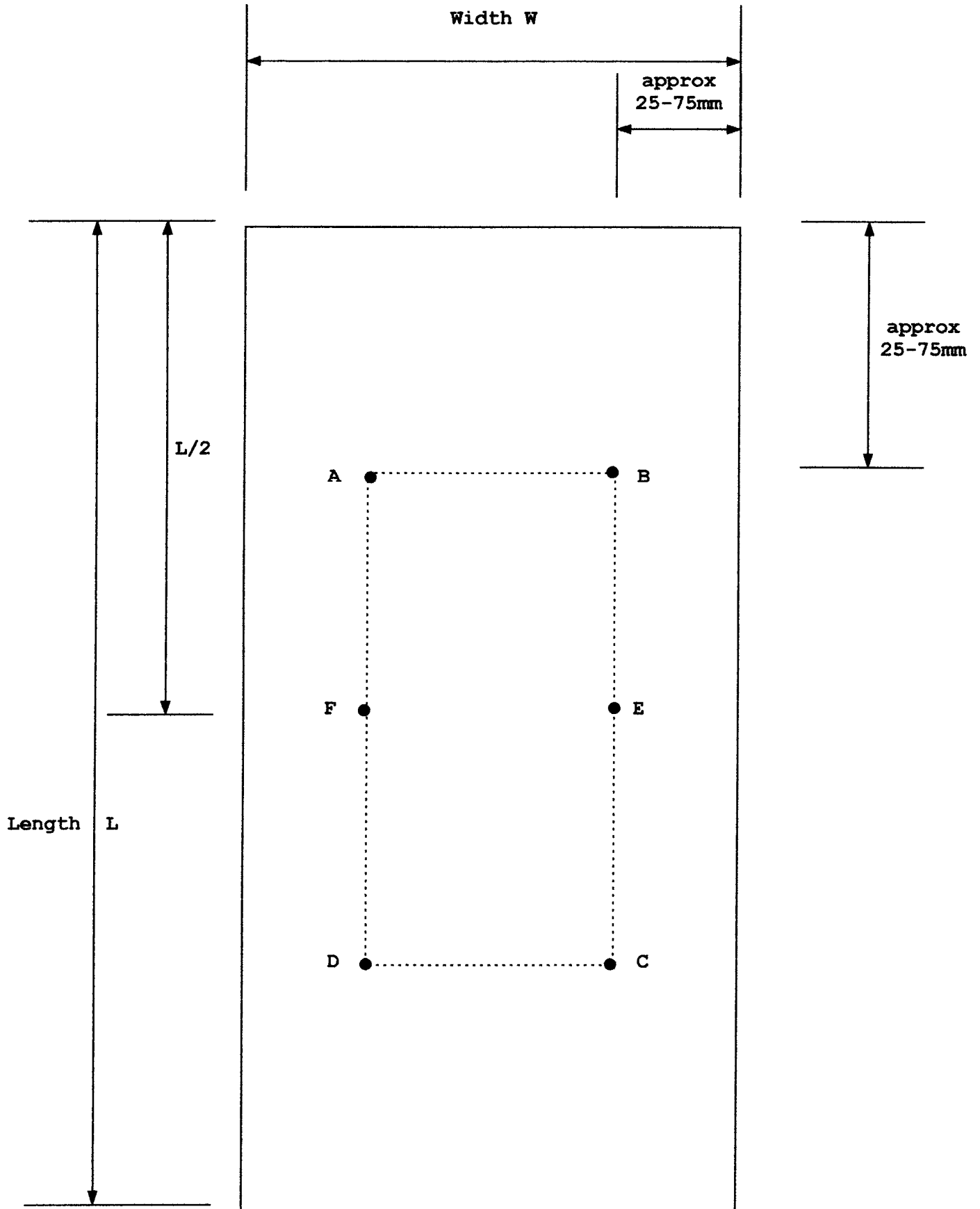
FIG. 1 Specimen Measurement
