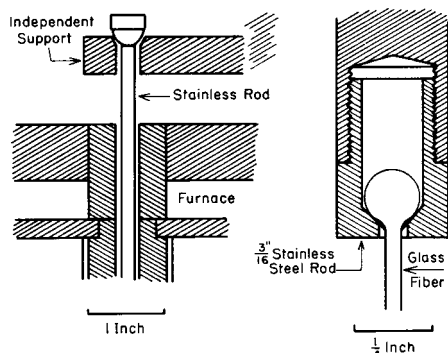
(a) Independent Support for Steel Rod (b) Method of Attaching Sample Fiber to Steel Rod.
