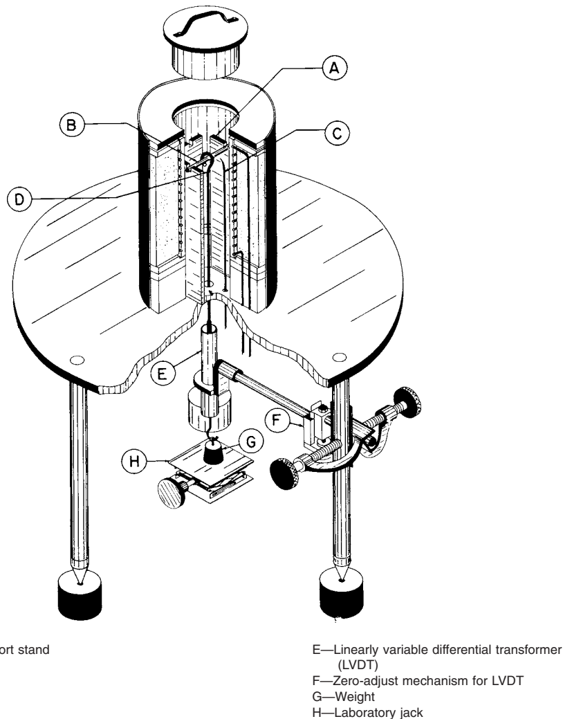
FIG. 1 Cutaway Drawing of Beam-Bending Apparatus
