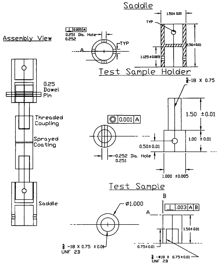
FIG. 1 Self-Aligning Device
