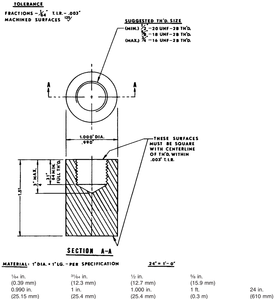
FIG. 2 Substrate and Loading Fixture
