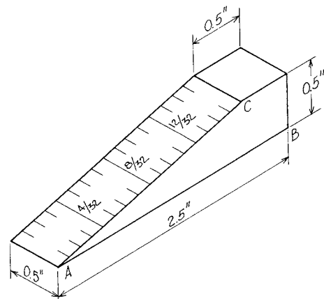
FIG. 1 Measuring Wedge
