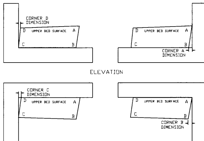
ELEVATION FIG. 4 Out-of-Square Measurements
