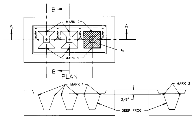
SECTION A-A SECTION B-B FIG. 3 Deep Froged Units
