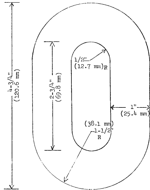
FIG. 4 Test Specimen
