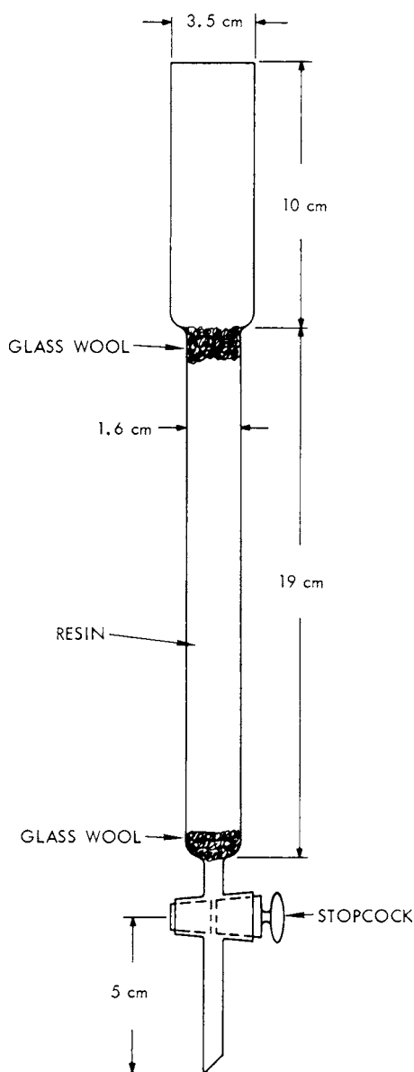
FIG. 8 Adsorption Column
