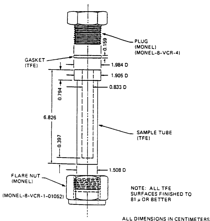
FIG. 2 Small TFCE Sample Tube
