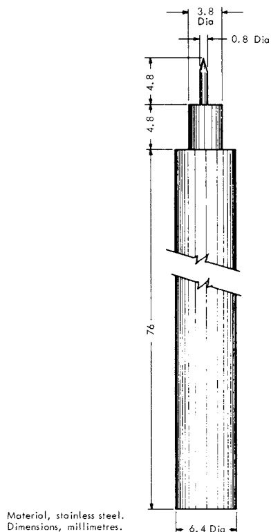
FIG. 7 Vent-Forming Tool
