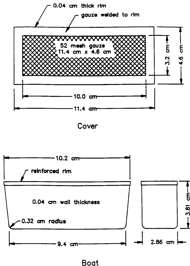
FIG. 5 Platinum Boat and Cover
