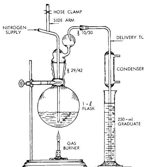
FIG. 6 Apparatus for Distillation of Chlorine
