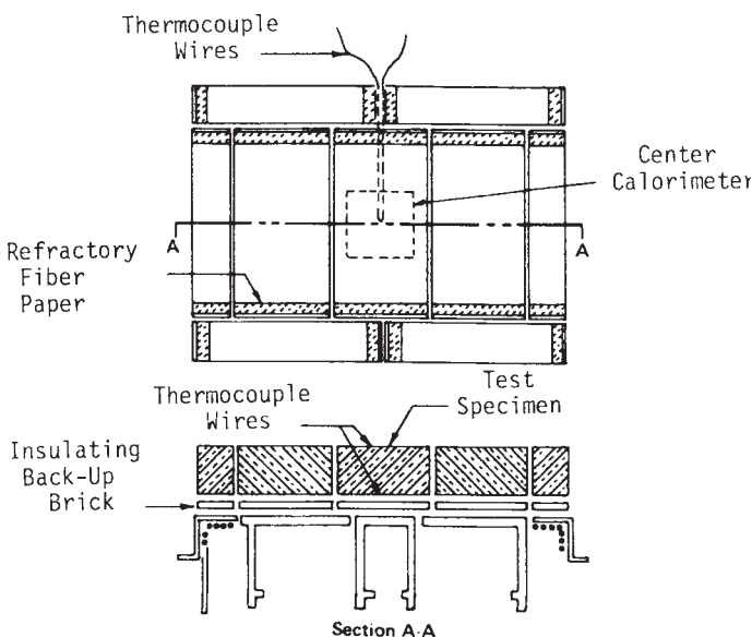
FIG. 1 Arrangement of Refractory-Fiber Paper Strips in Calorimeter Assembly
