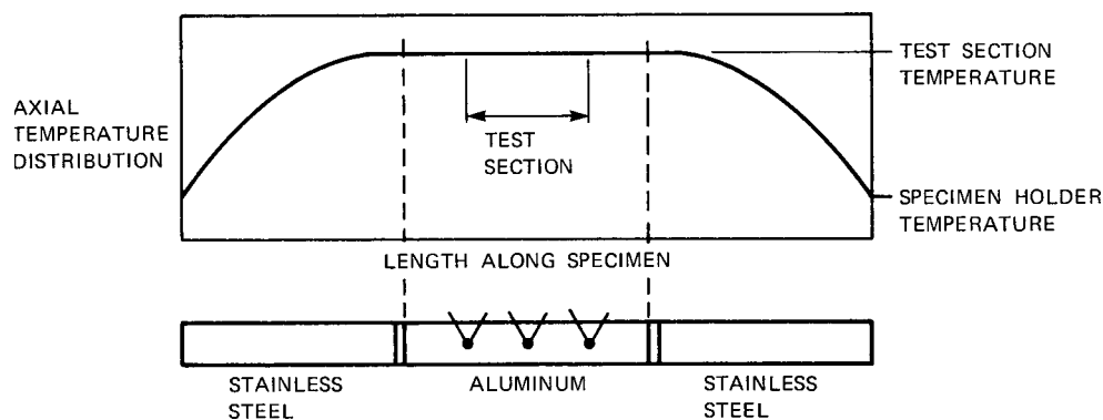
FIG. 8 Composite Specimen
