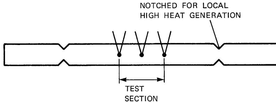
FIG. 9 Notched Specimen
