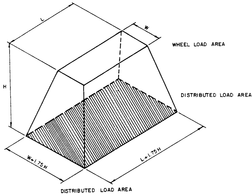
DISTRIBUTED LOAD AREA FIG. 3 Distributed Load Area
