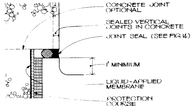
FIG. 2 Terminal Condition Above Finish Grade on Concrete Wall (see 8.3.1)
