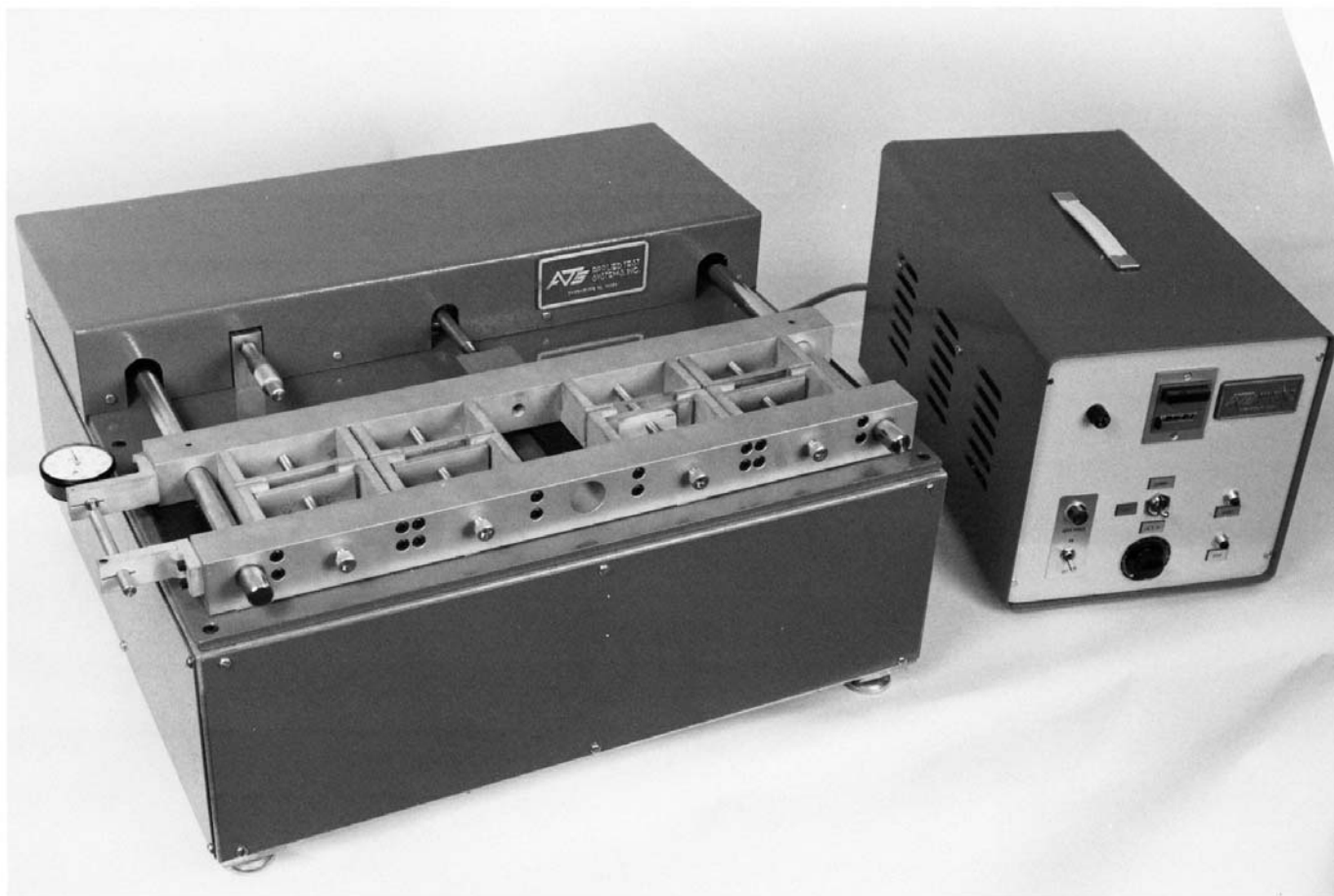
FIG. 1 Compression-Extension Machine
