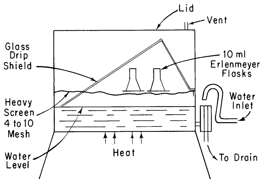
FIG. X1.1 Steam Chamber
