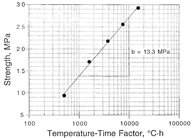
FIG. X1.1 Example Data of Strength as a Function of the Logarithm of the Temperature-Time Factor and the Best-Fit Straight Line that Represents the Prediction Equation
