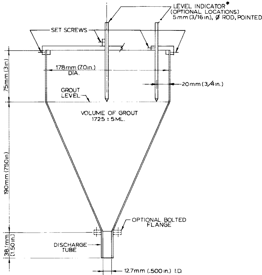
NOTE 1—Other means of indicating grout level may be used as long as accurate indication of grout level on volume is obtained. FIG. 1 Cross Section of Flow Cone
