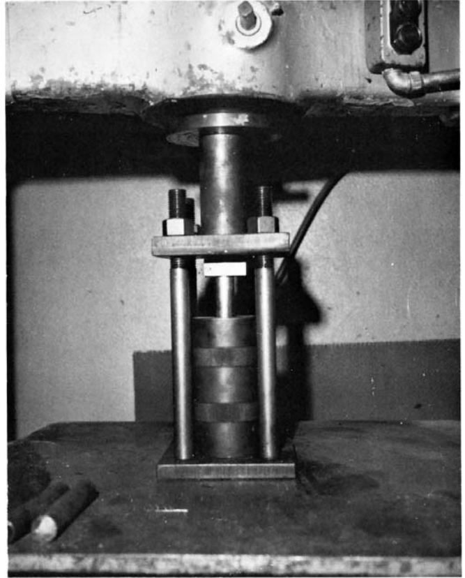
FIG. 3 A Typical Assembled Pressure Vessel
