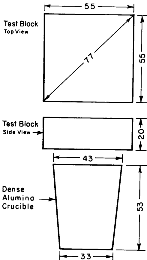
FIG. 1 Crucible-Cover Assembly
