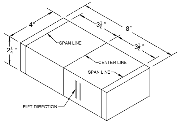
Specimen for Testing Parallel to Rift
