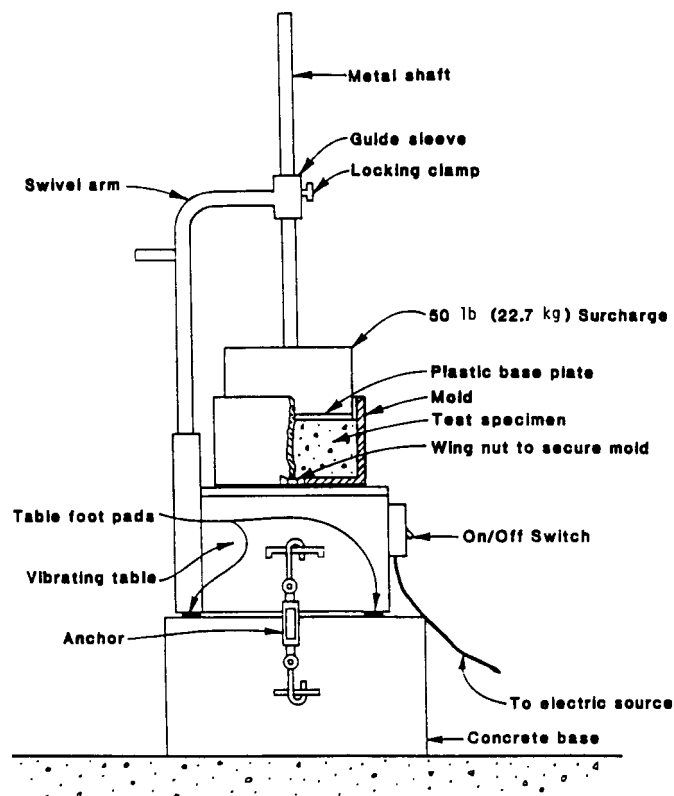
FIG. 1 Vibrating Table—Consistency Test (Test Method A)
