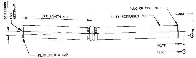
FIG. 1 Deflection Test (Plan View)
