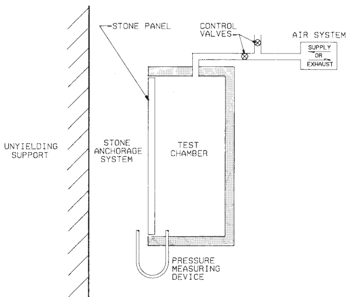
FIG. 1 General Arrangement of Testing Apparatus
