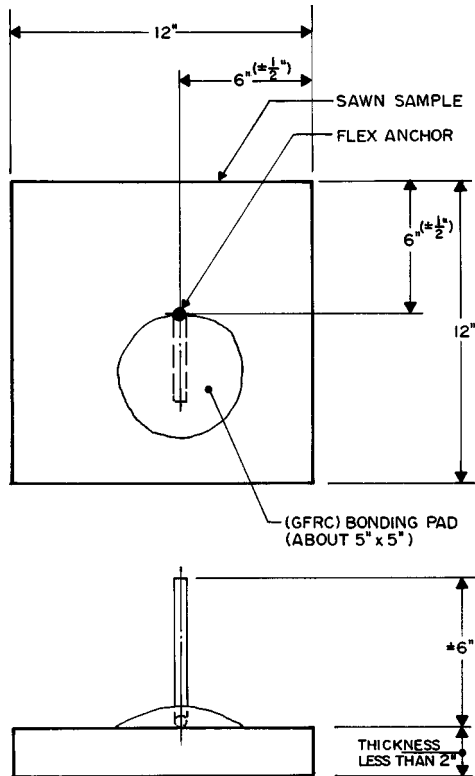
FIG. 4 Test Specimen
