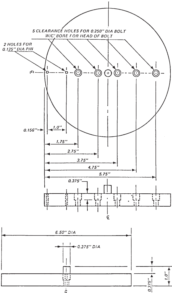
FIG. 3 Base Plate
