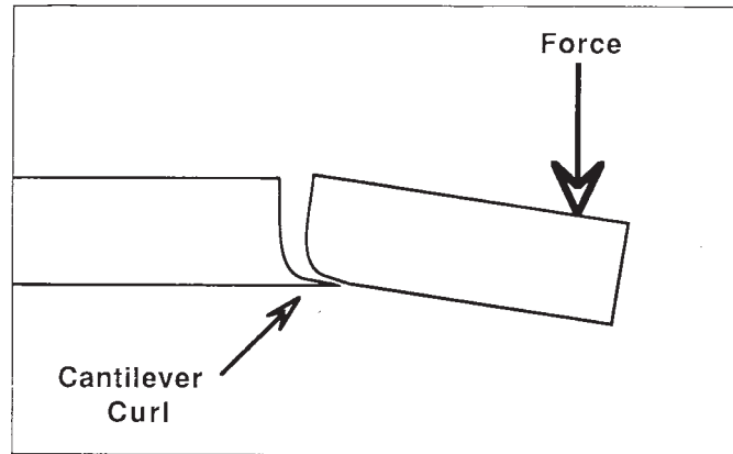
FIG. 13 Cantilever Curl, Formed on the Compression Side Under a Bending Stress
